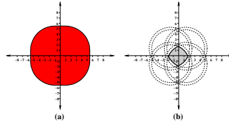
FIGURE 3: A decomposition of the constraint c_{a,r}(x) into c'_{a,r}(x) (left side) and -c''_{a,r}(x) (right side).
