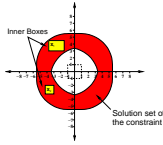
FIGURE 2: Some examples of inner boxes (boxes included inside the solution set of c_{a,r}(x) ).
