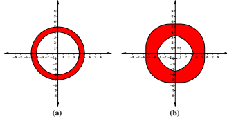
FIGURE 1: Two quantified distance constraints and their solutions. In (a), the distance \mathbf{r} = [4, 5] . In (b) the center \mathbf{a} = ([-1, 1], [-1, 1]) .
