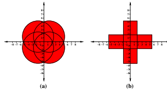
FIGURE 4: A description of c'_{a,r}(x) with (a) four constraints of the form f(x) \leq \bar{r} and (b) two inclusion constraints of the form \mathbf{x} \subseteq \text{box} .
